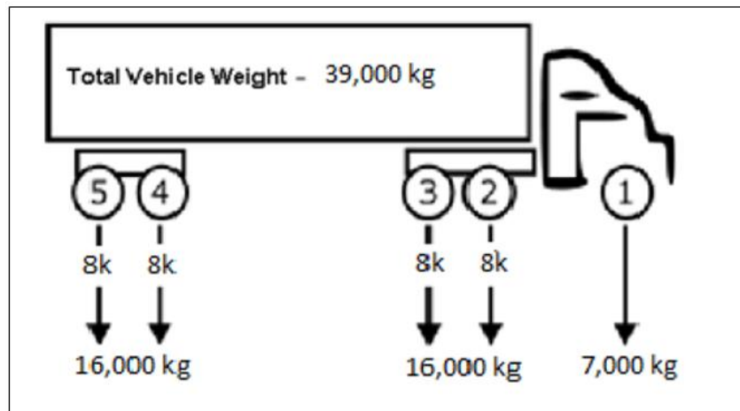
Figure 1: Wheeled Vehicle Specifications – Example
